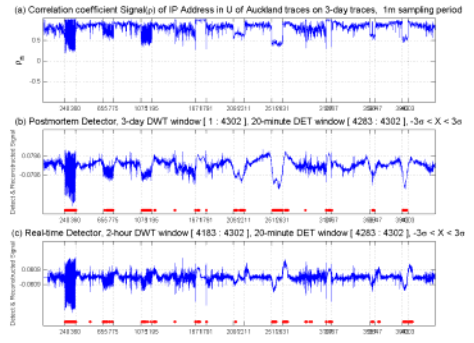
Fig. 3. The Univ. of Auckland detection results in postmortem and real-time mode
